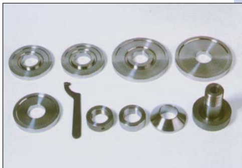
108963 Universal hubless / composite adapter
