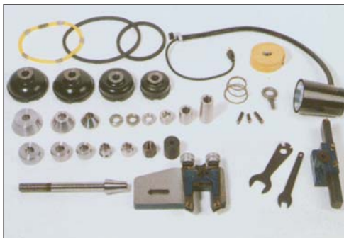
Complete tooling package for 201 TrueCut
